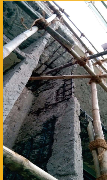
Structural Repairs
