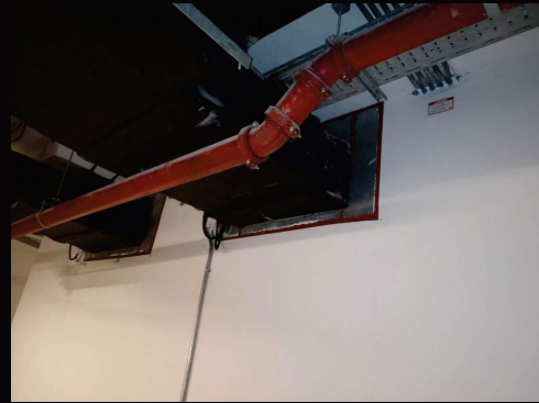
Firestopping for penetrations through wall
